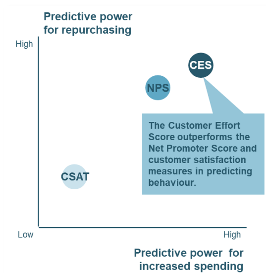
Fig. 8: Comparison of predictive power between CSat, NPS and CES according to the CES designers. Source: "Stop trying to delight your customers" (DIXON, FREEMAN, & TOMAN, 2010)
